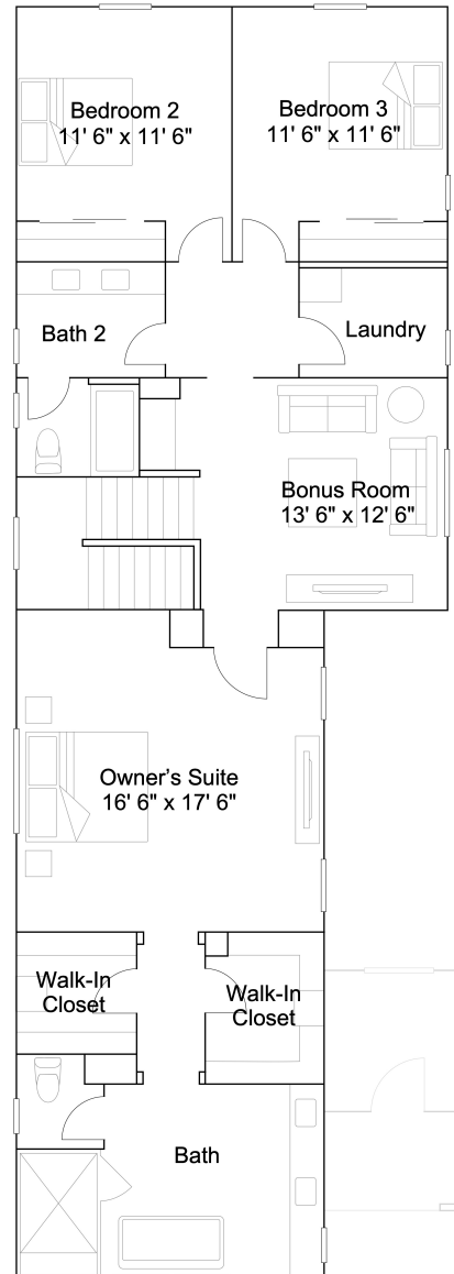
SECOND FLOOR
