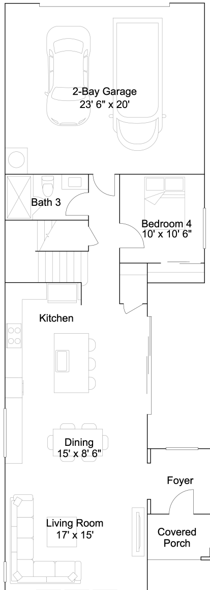
FIRST FLOOR
