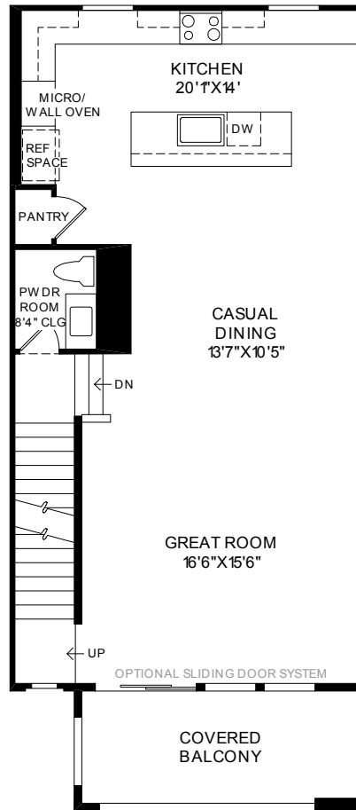
SECOND FLOOR 9' CEILING HEIGHT
