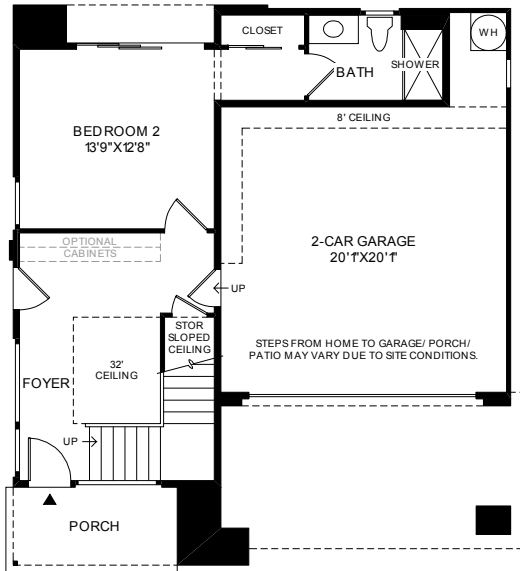
FIRST FLOOR 9' CEILING HEIGHT
