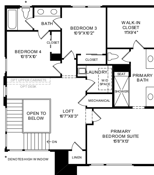
THIRD FLOOR 10' CEILING HEIGHT
